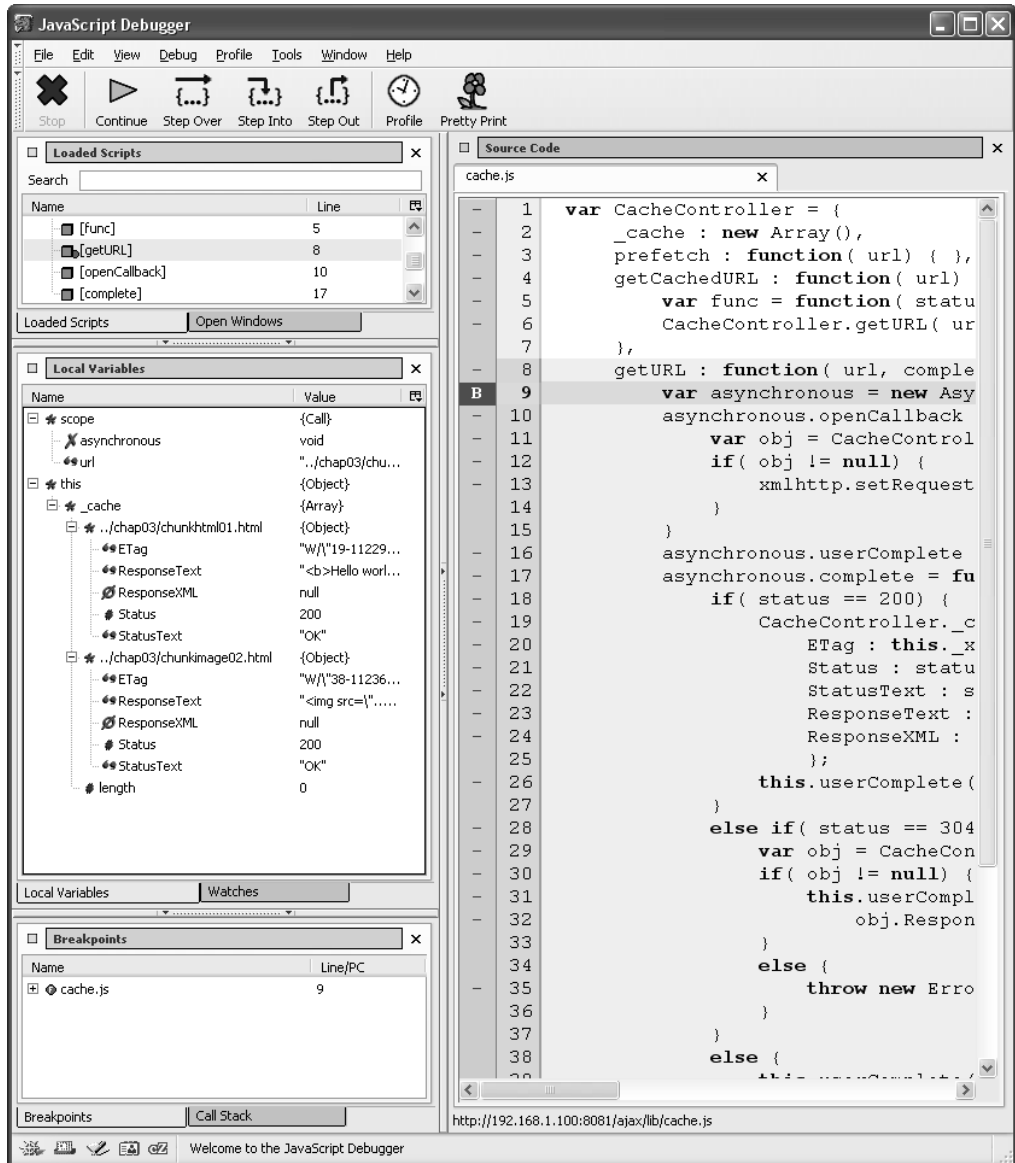
Figure 4-4. Mozilla debugger illustrating that there are two items in the cache
