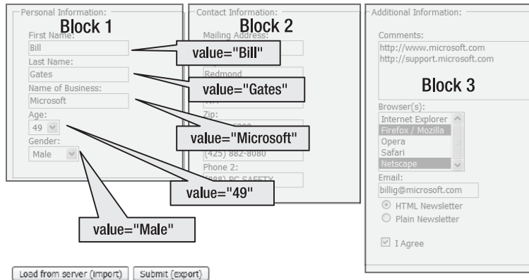
Figure 7-8. Example HTML form converted into three state blocks
