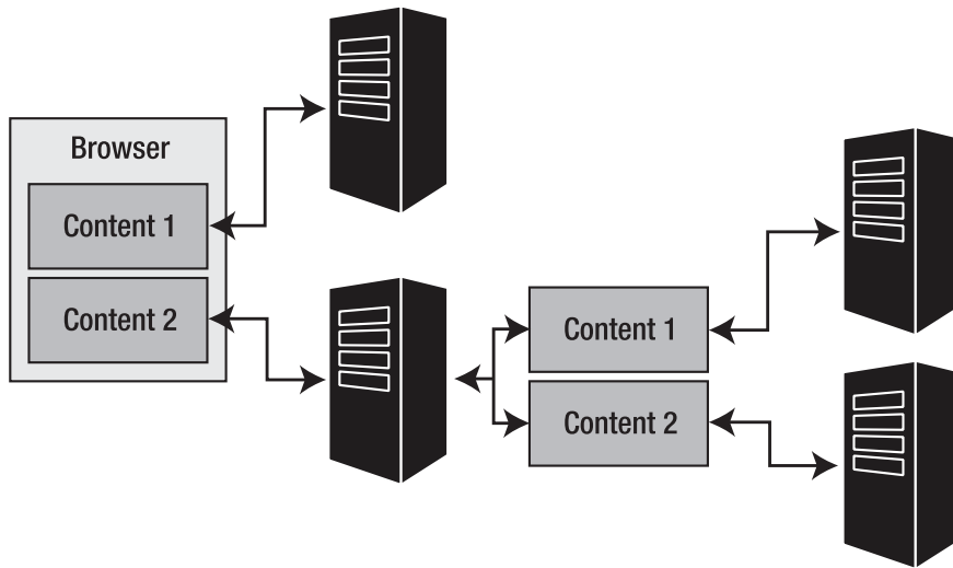
Figure 1-9. Ajax architecture
