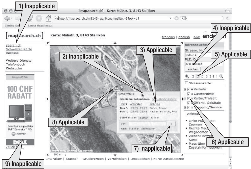
Figure 6-5. Applicable and not applicable scenarios of the Decoupled Navigation pattern
