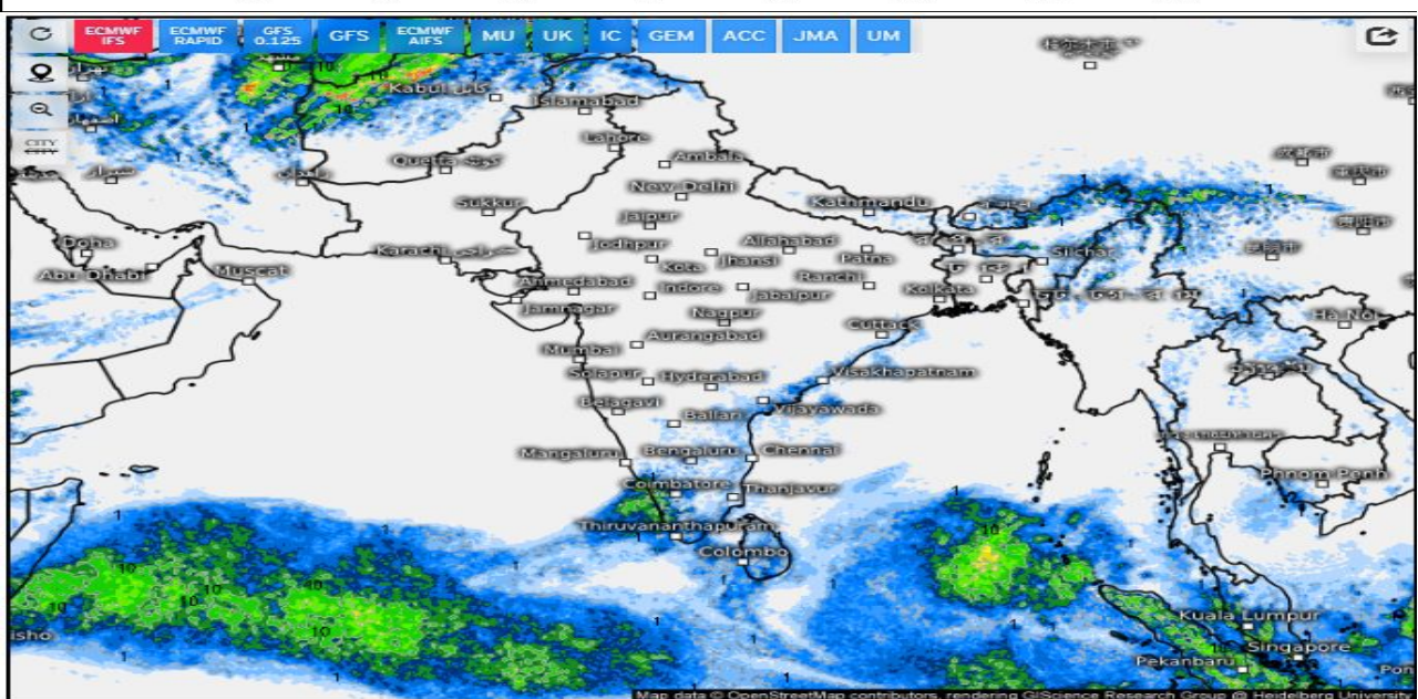
Precipitation, 24h (mm) i Valid for Tue 03/25/2025, 05:30am IST
