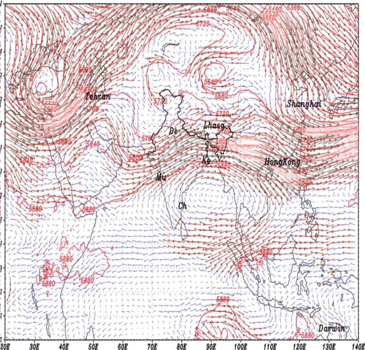
NCUM ANALYSIS VALID ON 00Z20MAR2025 500 hPa GEOP(m) & WINDS(m/s)
