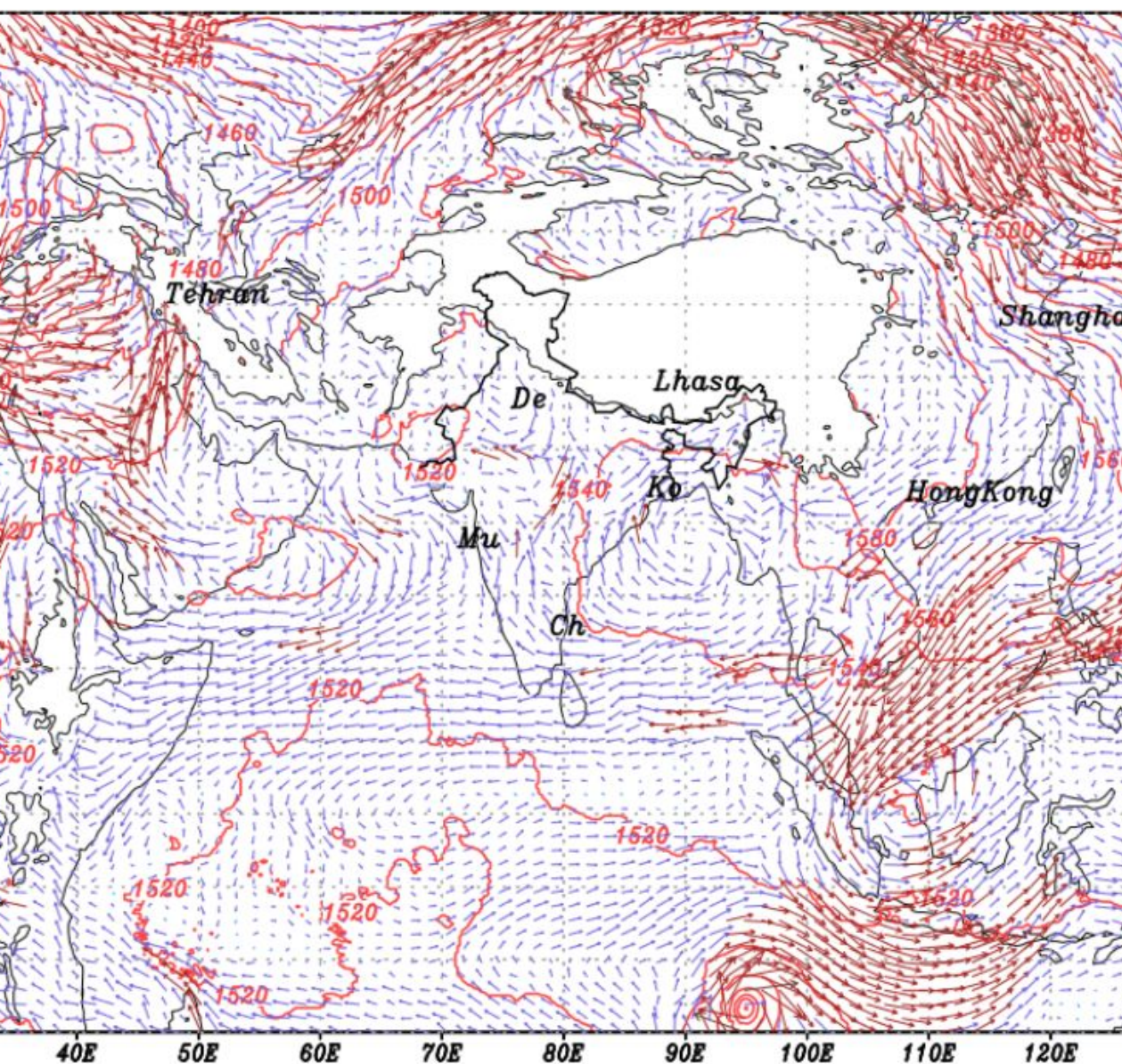
NCUM ANALYSIS VALID ON 00Z20MAR2025 850 hPa GEOP(m) & WINDS(m/s)
