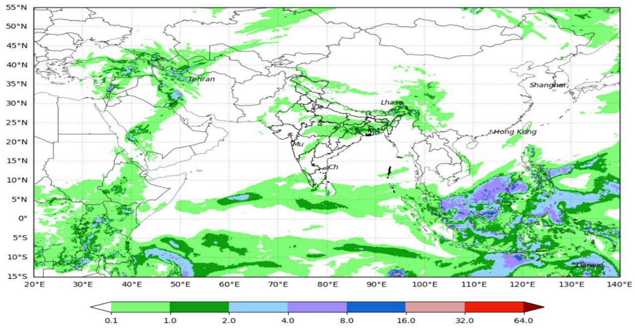
NCUM 24HR FORECAST VALID ON 03Z21Mar2025 RAINFALL(cm) CI=0.1,1,2,4,8,...
