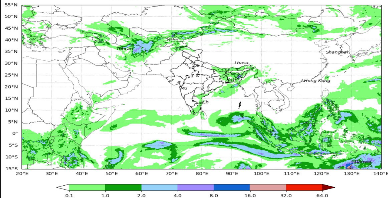
NCUM 120HR FORECAST VALID ON 03Z25Mar2025 RAINFALL(cm) CI=0.1,1,2,4,8,...
