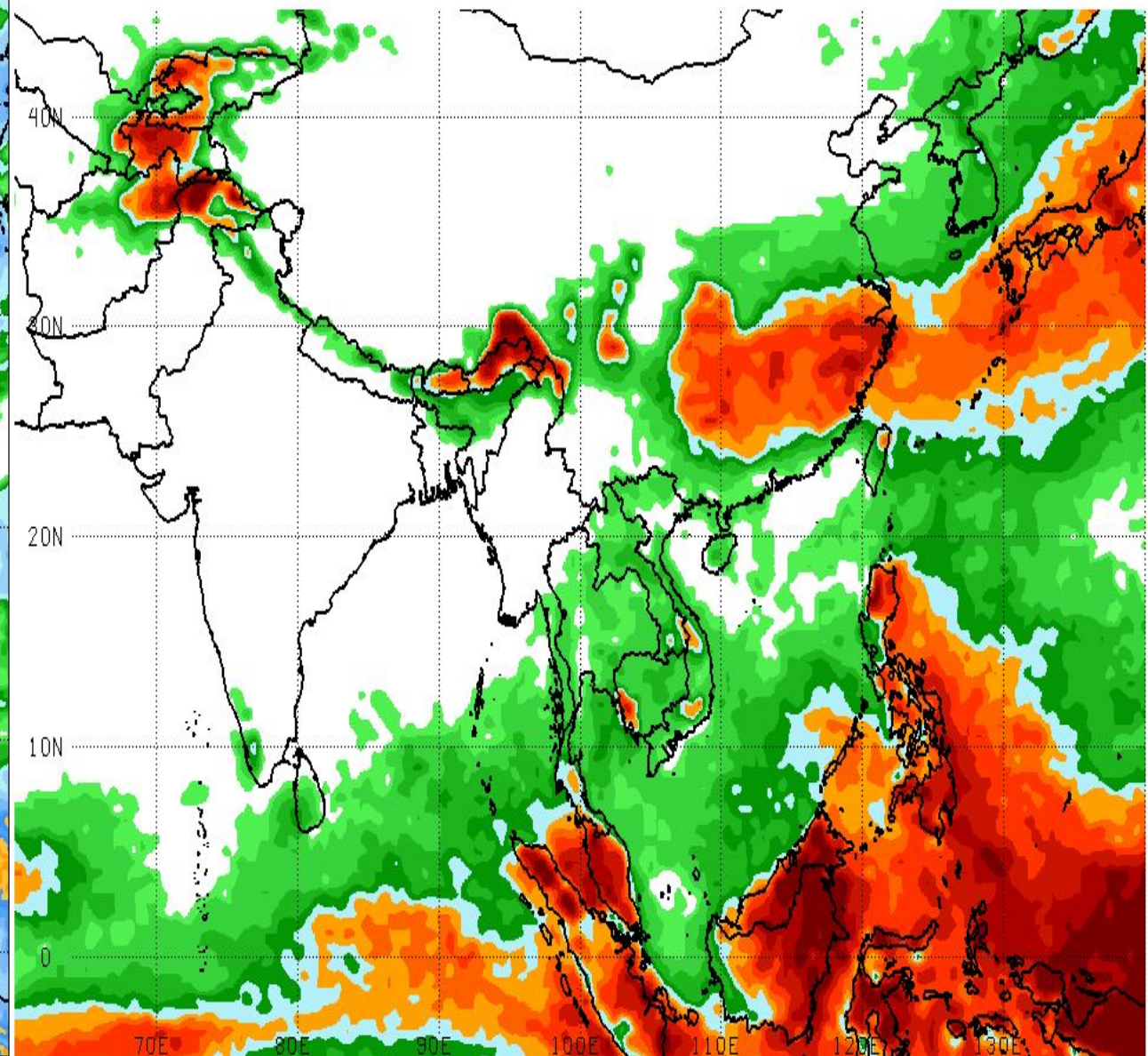
NOAA GEFS 20250319 00zCYC FCST Probability of Week2 Precip > 25mm VALID 20250402/0000V336
