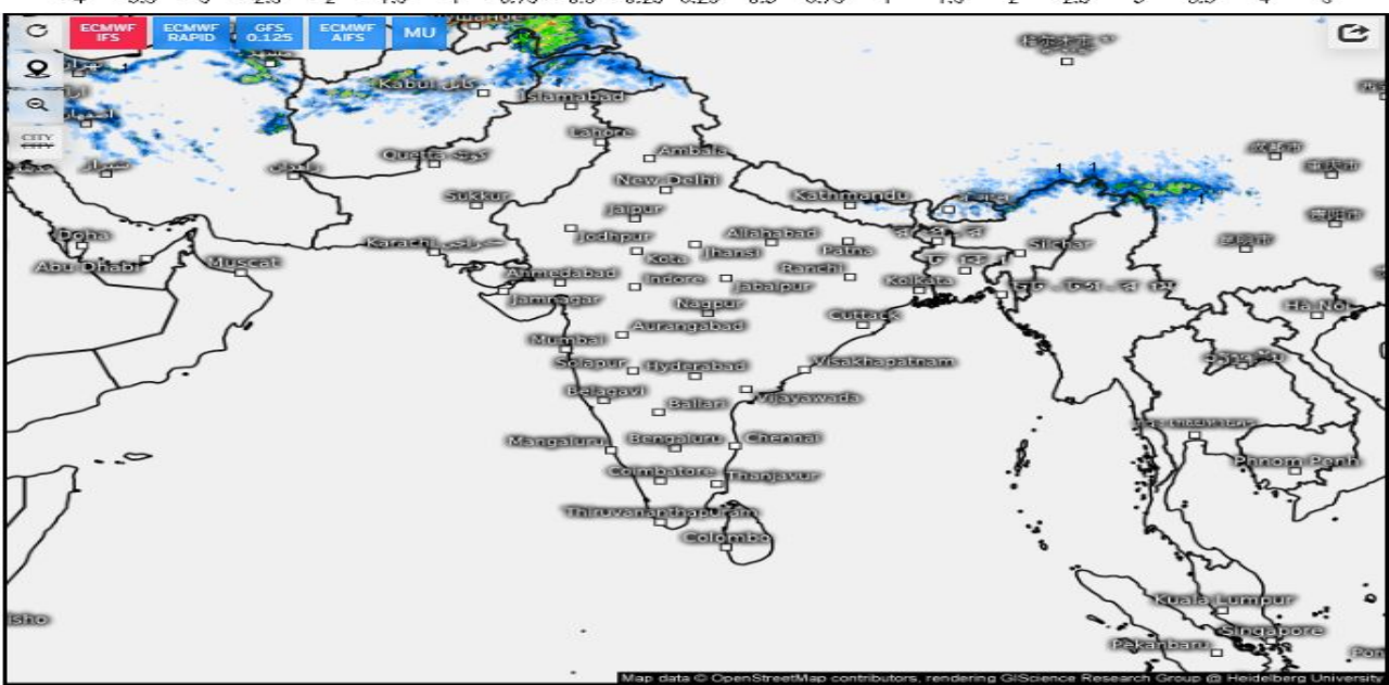
Precipitation, 24h (Snow) (mm) i Valid for Tue 03/25/2025, 05:30am IST
