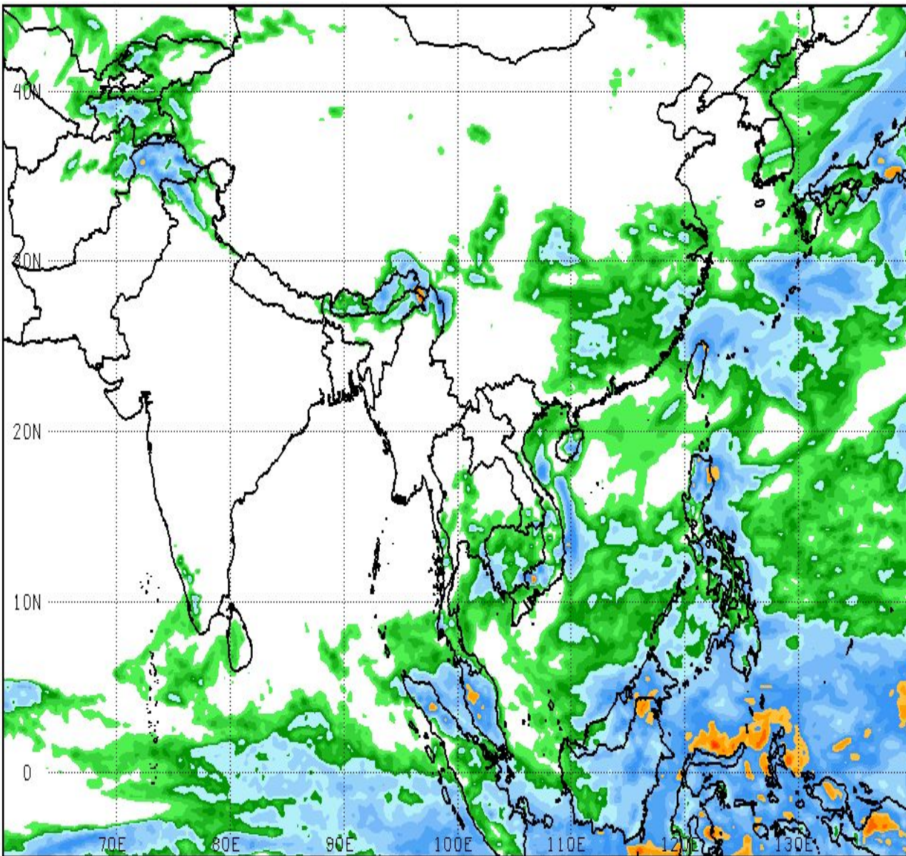
NOAA GFS 20250319 t00z cycle FCST week2 Total Precip (mm) VALID 2025040200Z
