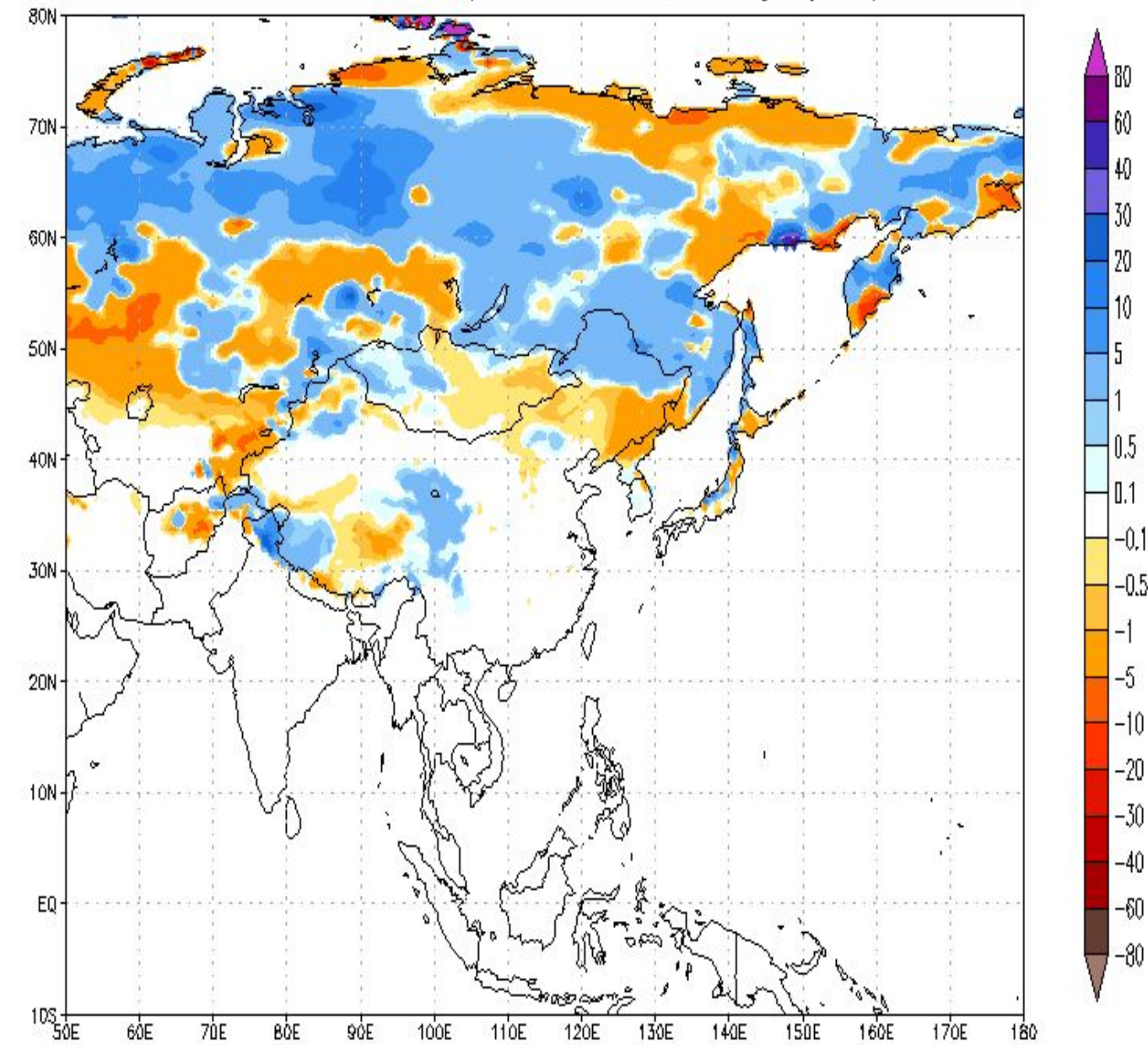
Calculated Snow Water Equivalent Anomaly (cm) 20250318
