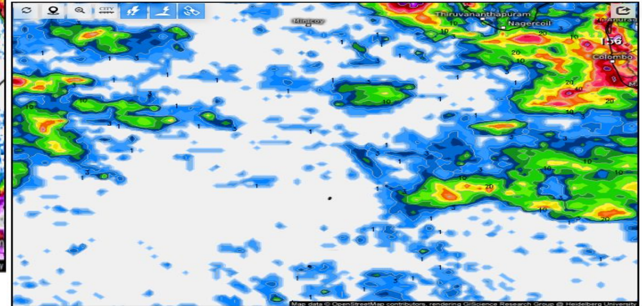
Accumulated Precipitation, 7 days (Satellite) (mm)
