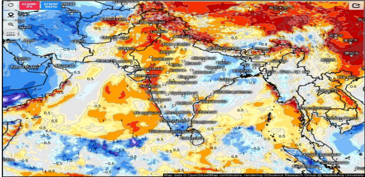
Temperature anomaly (std. deviation) i Valid for Tue 03/25/2025, 02:30pm IST
